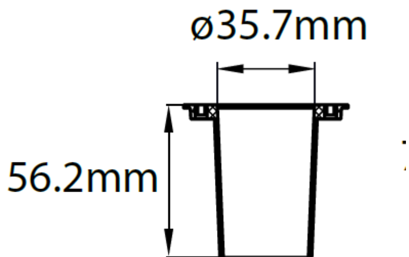
Housing H035
