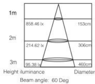
Lux- distance curve
