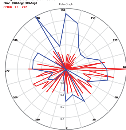
2D Light Intensity Distribution Curve Plane [50%Ang][10%Ang] C110.0: 7.5 73.2
