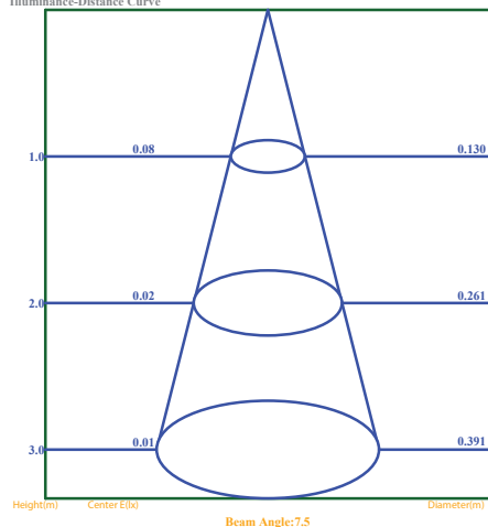
Illuminance-Distance Curve
