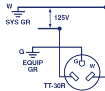
Wiring Diagram
