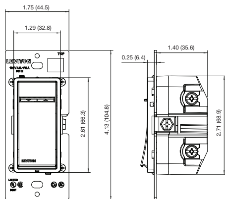
VRI06-1L
