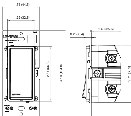
VRS15-1L VRS05-1L
