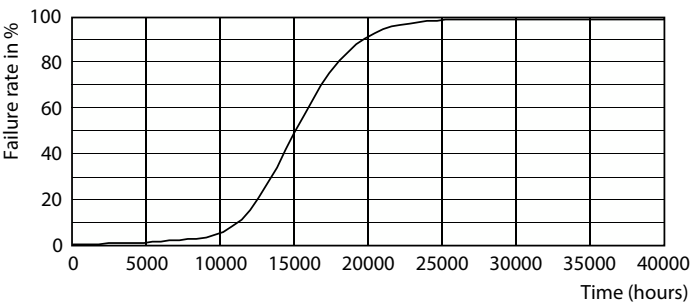
Life Expectancy Diagram - Ess LEDBulb 8-60W E27 6500K 1PF/6 MX
