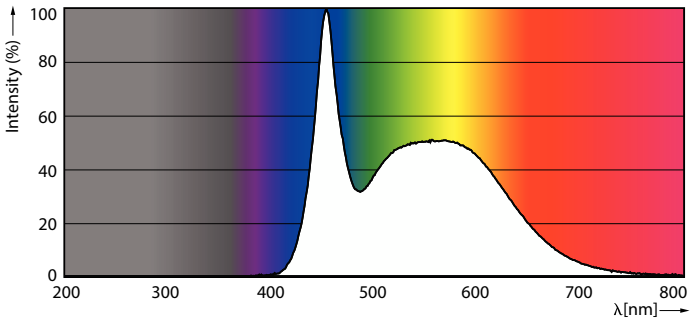
Spectral Power Distribution Colour - Ess LEDBulb 8-60W E27 6500K 1PF/6 MX
