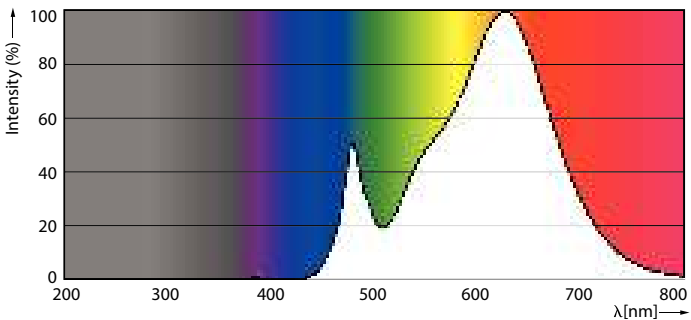
Spectral Power Distribution Colour - ESS LEDBulb 12-100W E27 3000K 1PF/6 MX
