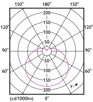
Light Distribution Diagram - ESS LEDBulb 12-100W E27 3000K 1PF/6 MX
