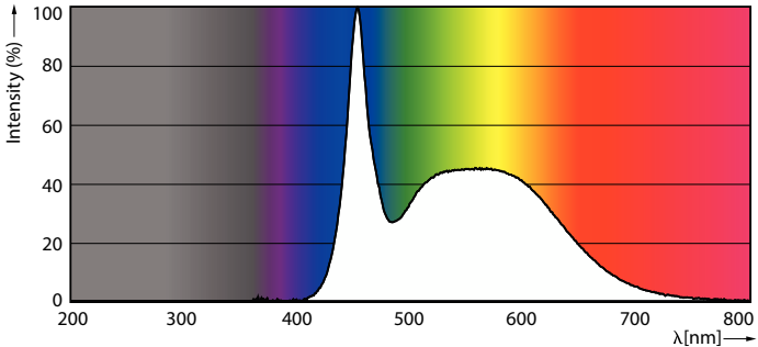
Spectral Power Distribution Colour - LEDspot 4-50W GU10 865 100-240V 36D ND
