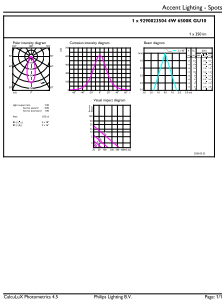
Accent Lighting Spots - LEDspot 4-50W GU10 865 100-240V 36D ND
