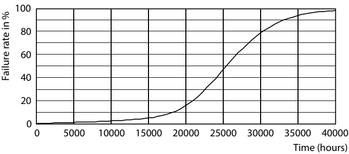
Life Expectancy Diagram - LEDspot 4-50W GU10 865 100-240V 36D ND
