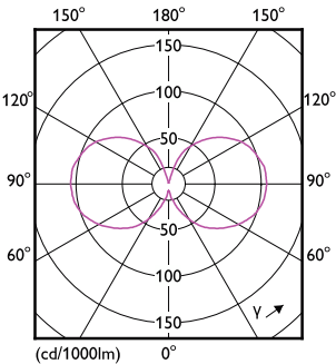
Light Distribution Diagram - LEDClassic 4.5W B11 E12 827 CL ND 1PF/10
