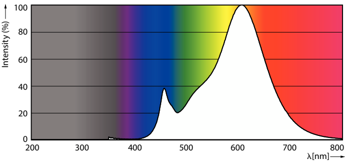
Spectral Power Distribution Colour - LEDClassic 4.5W B11 E12 827 CL ND 1PF/10
