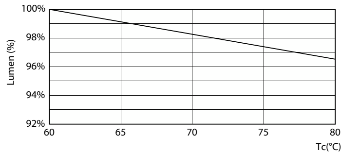
Lumen Maintenance Diagram - CorePro LEDtube HO 1200mm 18W840 VWV T8
