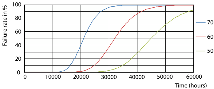
Life Expectancy Diagram - CorePro LEDtube HO 1200mm 18W840 VWV T8
