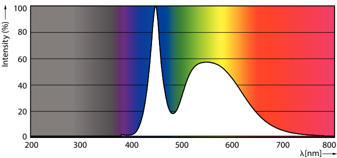
Spectral Power Distribution Colour - ECOFIT E LEDtube 1200mm 16W 765 T8 WV
