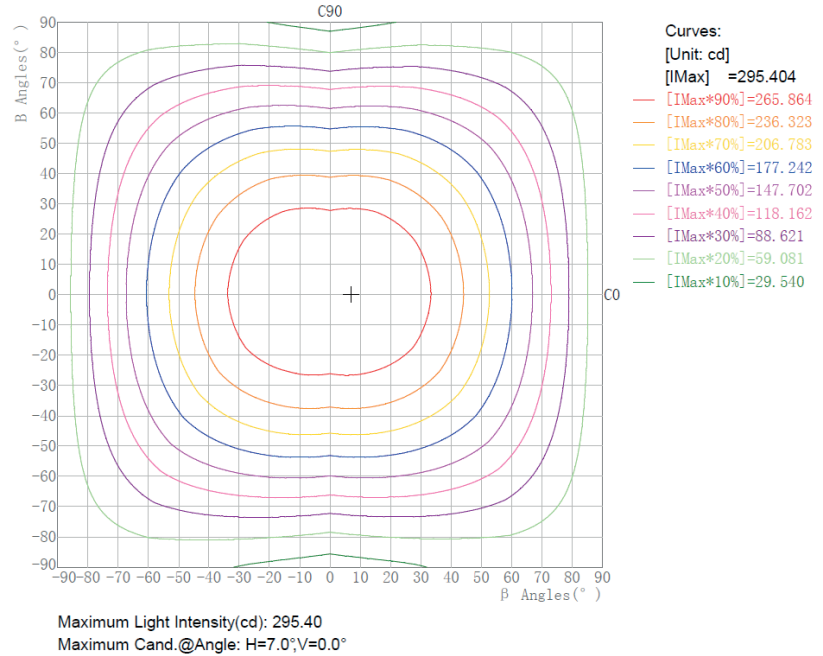
ISO Lighting Intensity Curve
