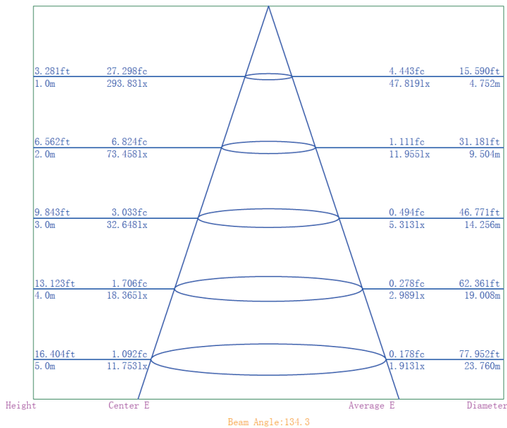
Illuminance-Distance Curve
