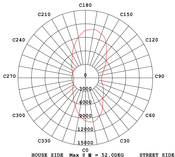
MAX INTENSITY CONE SURFACE DISTRIBUTION DIAGRAM
